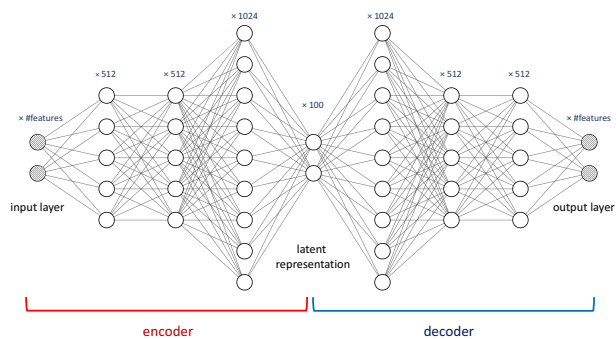
Fig. 1: The autoencoder (AE and VAE) architecture.
